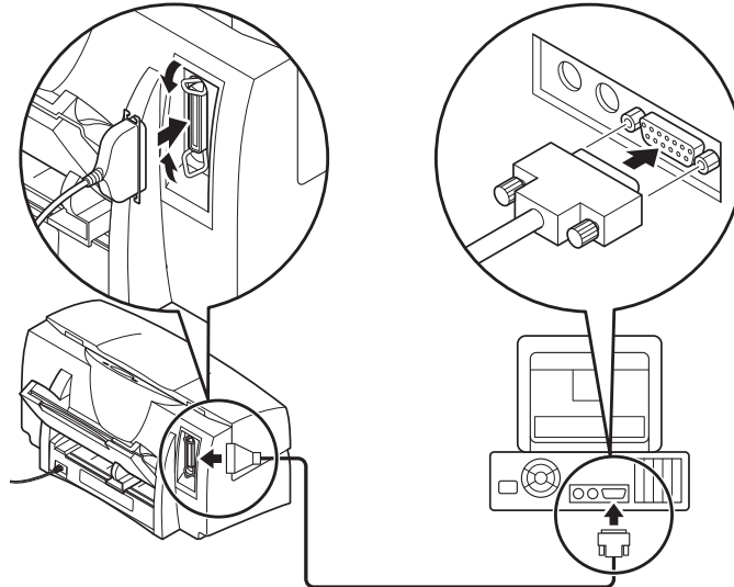
Figure 3-3 Connecting the Interface Cable
