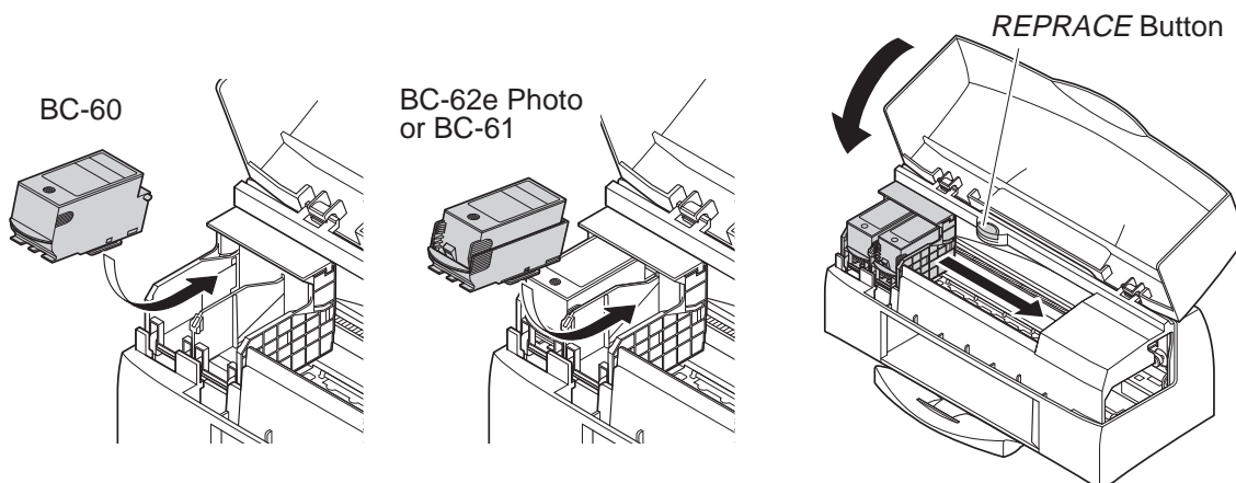
Figure 3-6 Installing BJ Cartridges
