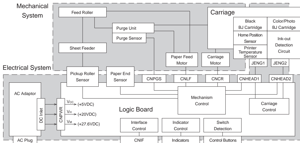
Figure 4-31 Printer Block Diagram
